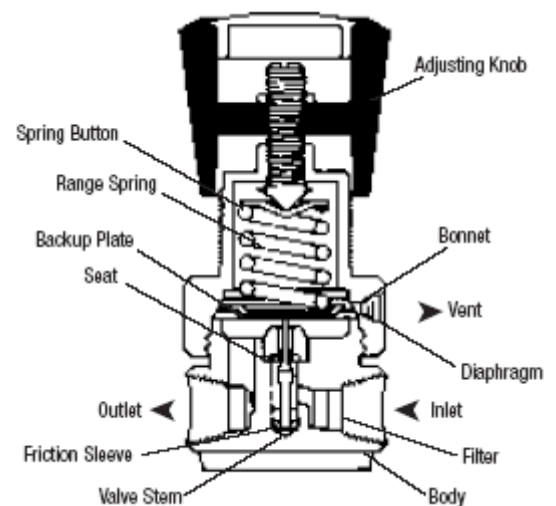
Figure 1 Single-stage regulator
